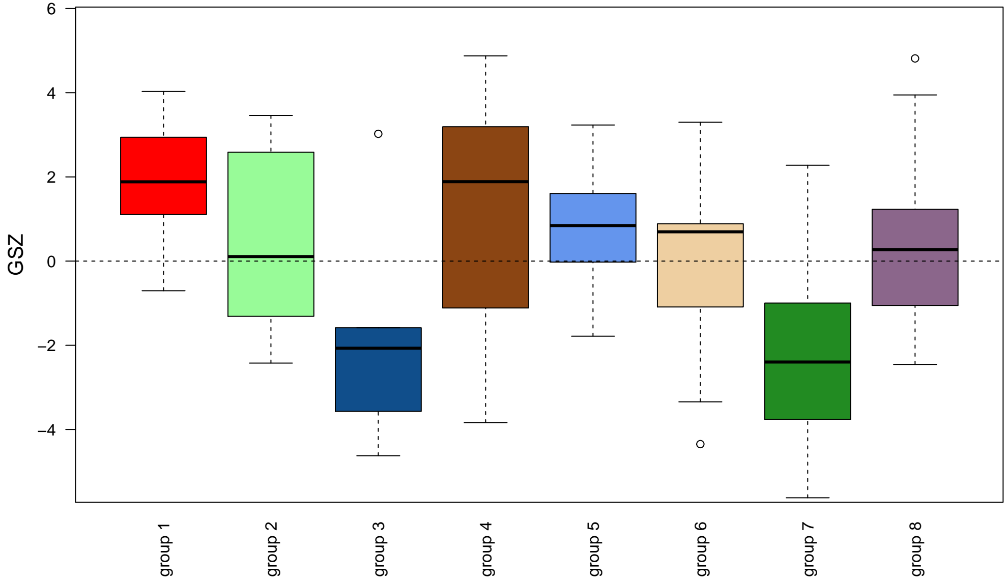
response to wounding
